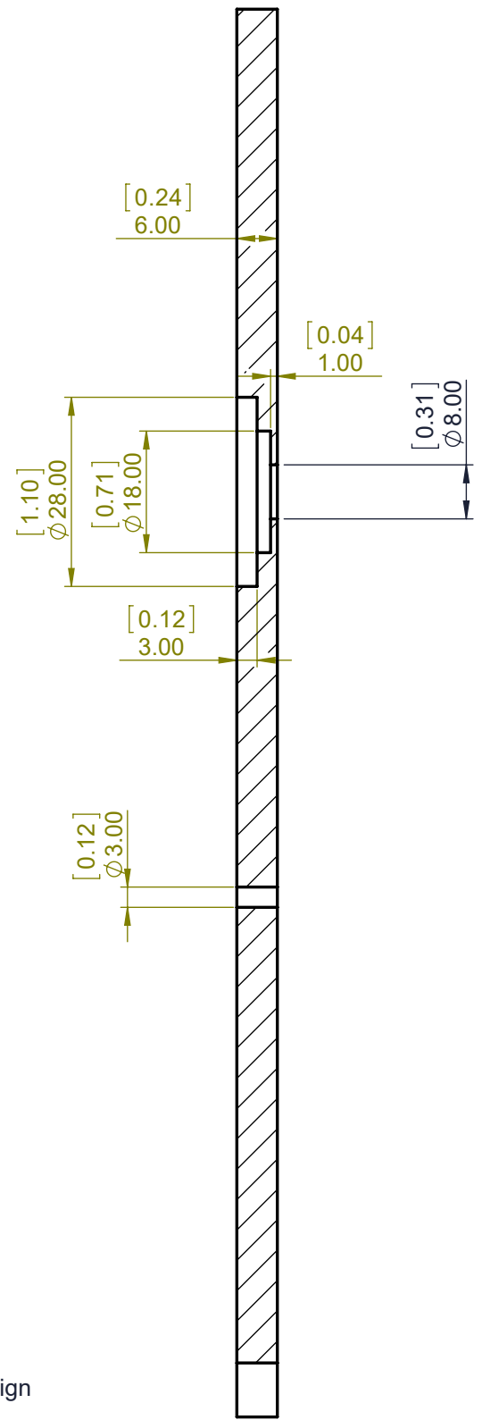
SECTION P-P
