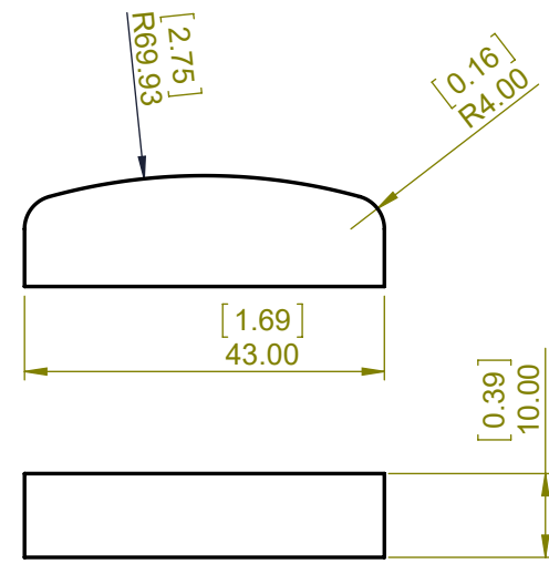
Dial Support wood 10 mm thick 2 Required Scale 1:1
